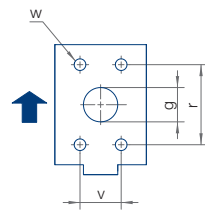
Pressure port (P)
